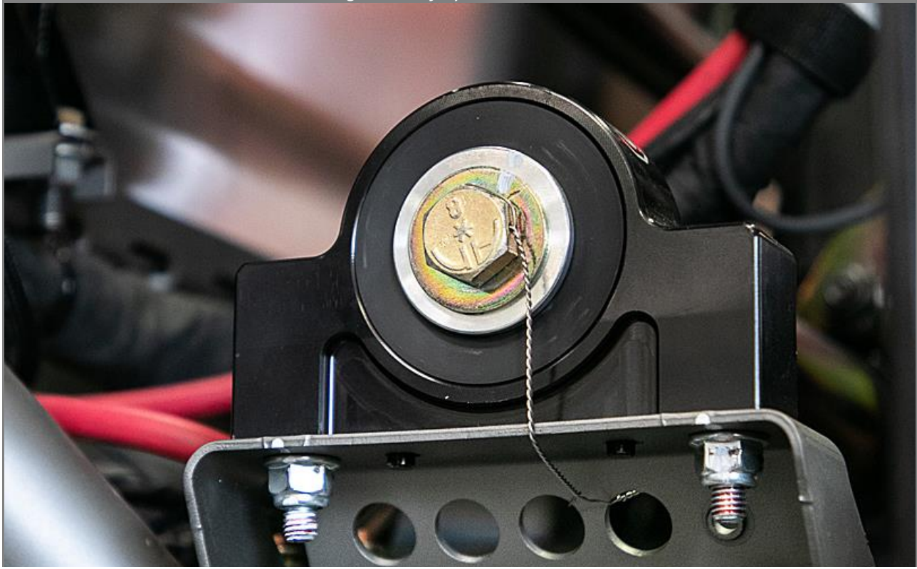
Figure 1: Safety-Wire Installed
